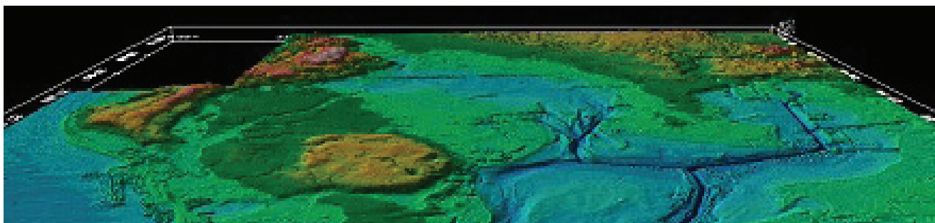
Coastal digital elevation models help determine how storm surge will affect an area.
